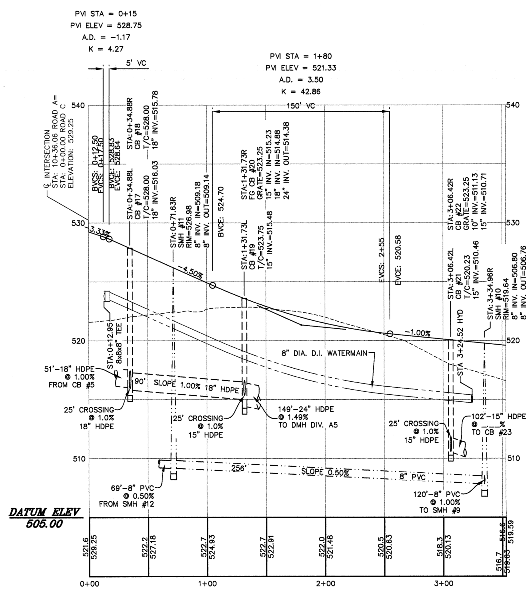
PROFILE: PROPOSED WILLIAM COURT SCALE: HORIZONTAL 1"=50' VERTICAL 1"=5'
