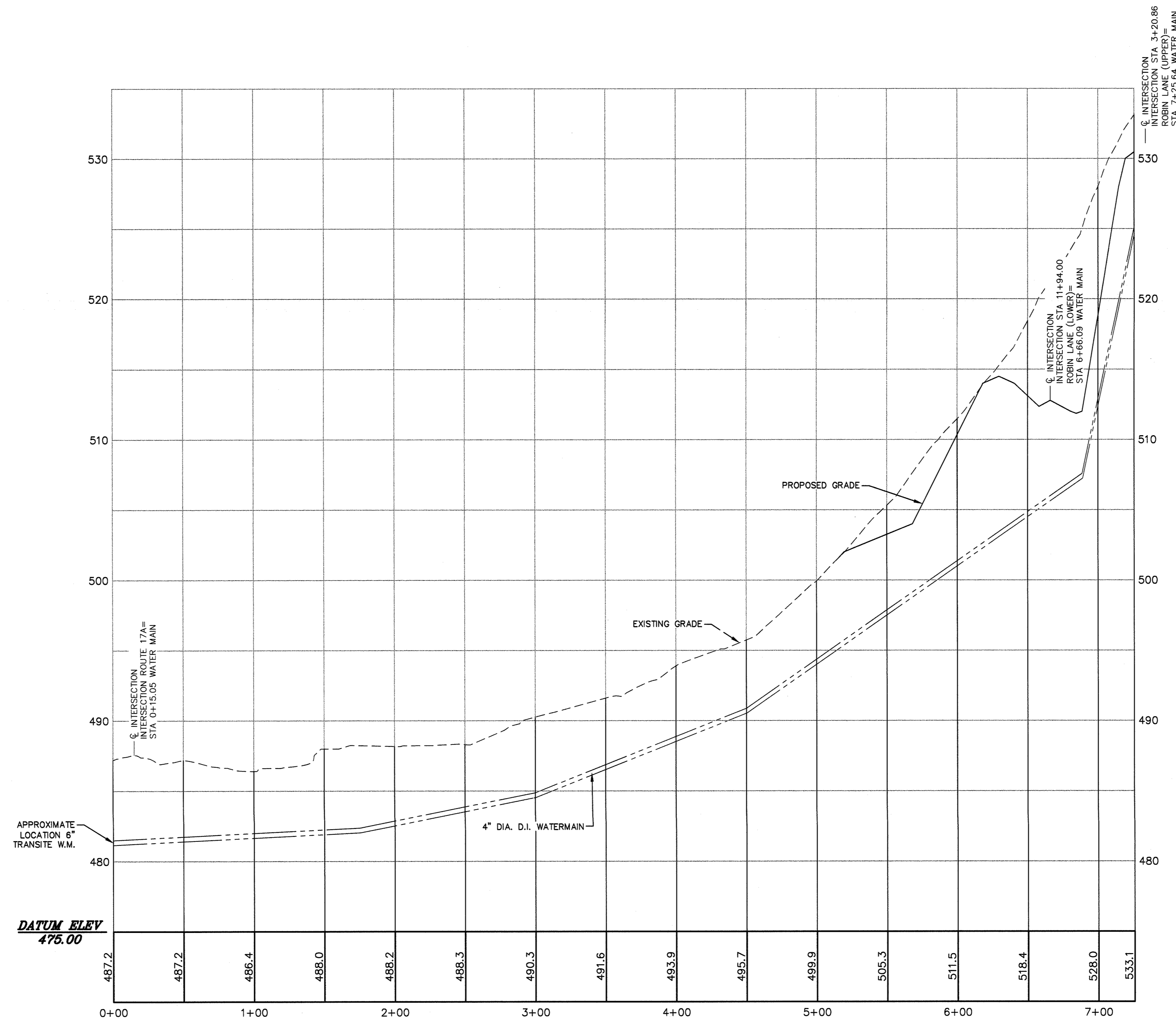
PROFILE: PROPOSED WATER MAIN RUN: NYS ROUTE 17A TO ROBIN LANE SCALE: HORIZONTAL 1"=50' VERTICAL 1"=5'
